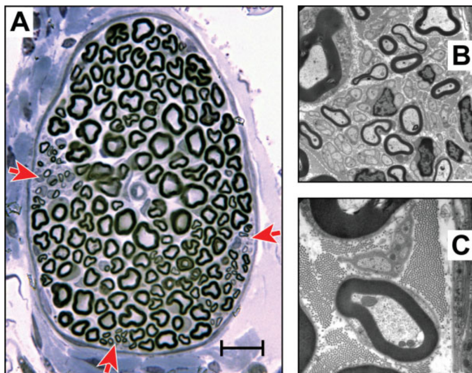
Fig. 1. (A) One-micron plastic section visualized under light microscope of a toluidine blue-stained recurrent laryngeal nerve cross-section of normal rat. Red arrows point to less myelinated and some unmyelinated axons as well. Scale bar is 50 \mu m. Electron micrographs of normal recurrent laryngeal nerve cross-section showing myelinated and unmyelinated axons and Schwann cells at original magnifications of (B) \times 15,000 , and (C) \times 45,000 .
